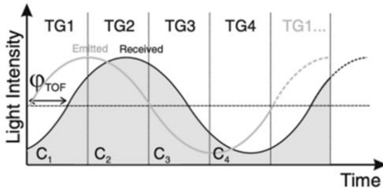
Figure 2-1. Light flight time vs. light intensity
