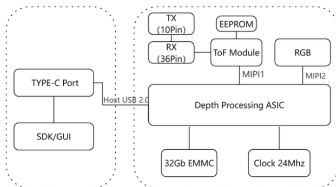
Figure 2-2. CS30 RGBD Camera System Frame Diagram
